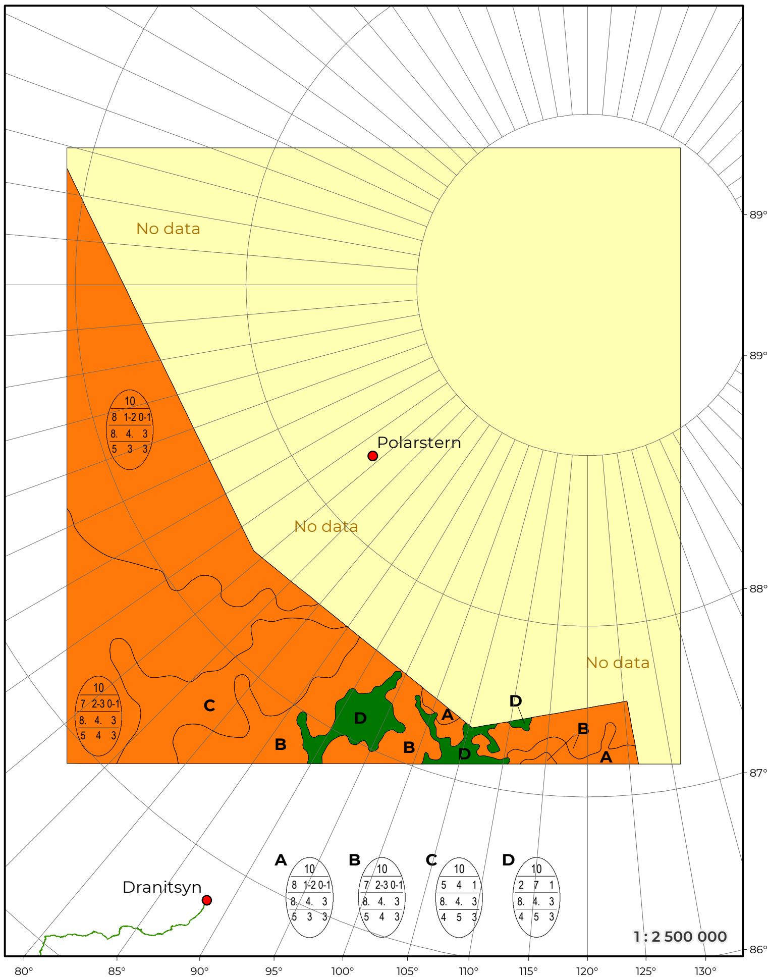
Arctic Ocean (Sectors of Barents, Kara and Laptev Seas) Detailed ice chart February 20, 2020
